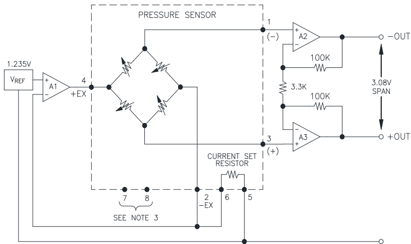
APPLICATION SCHEMATIC
