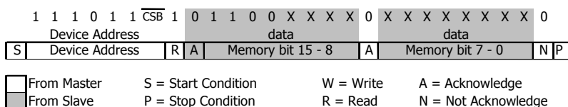
Figure 12: I 2 C answer from MS5607-B
