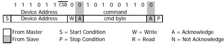
Figure 13: I 2 C Command to read memory address= 011 (Coefficient 3)
