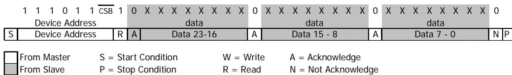
Figure 12: I 2 C pressure response (D1) on 24 bit from MS5803-01BA07
